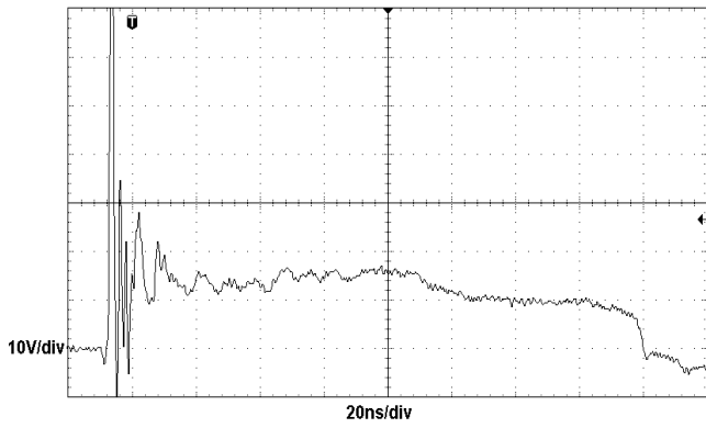
Fig.7 ESD clamping (+8kV contact discharge per IEC61000-4-2)
