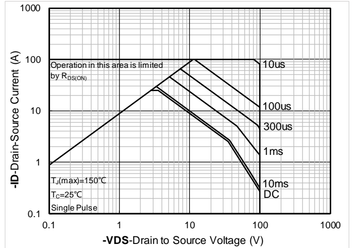
Figure8.Safe Operation Area
